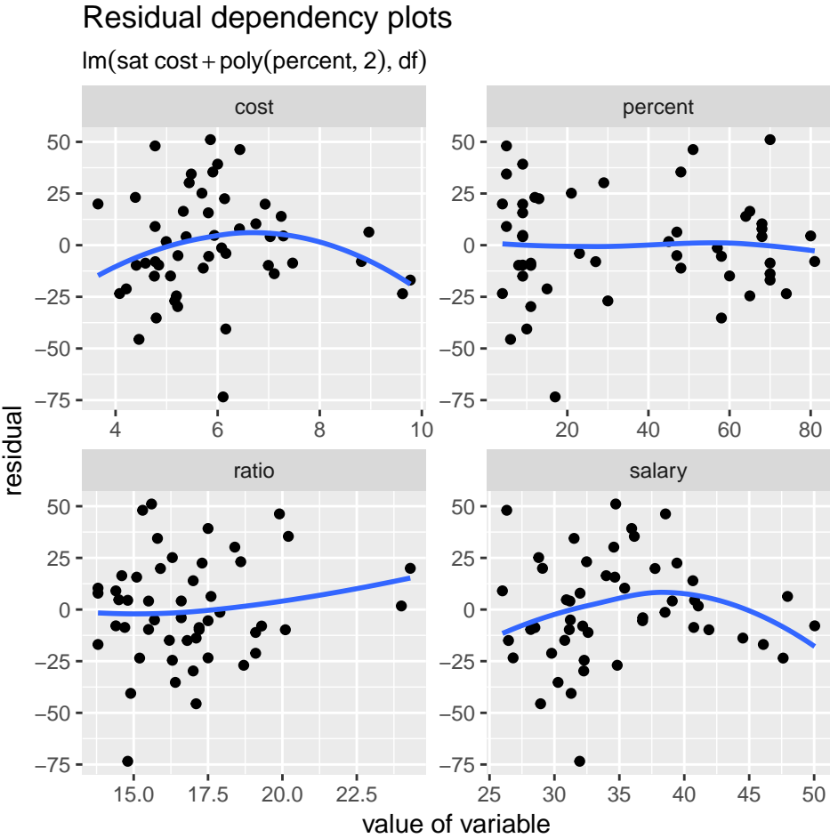
Figure 7: Residual Dependency Diagnostic Checks, Revised Model.
