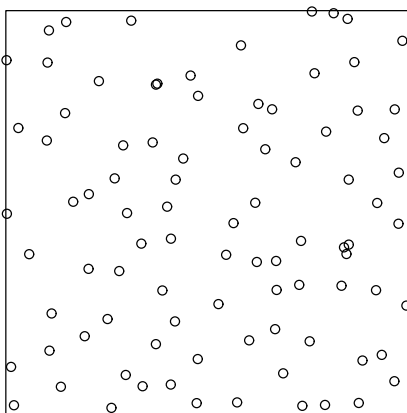
Strauss( \gamma=0.2 )
