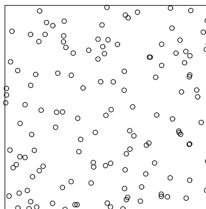
Strauss( \gamma=0.7 )
