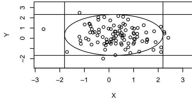
Correlation 0
