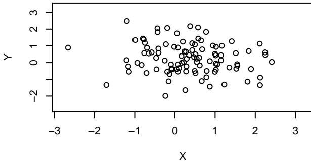
Correlation 0
