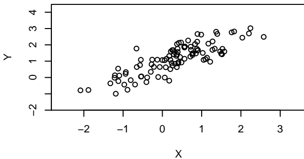
Correlation 0.9
