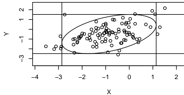
Correlation 0.45
