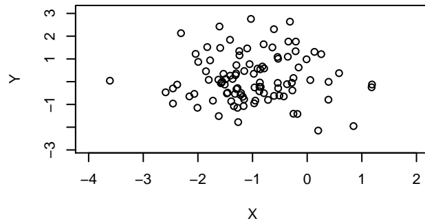
Correlation ??
