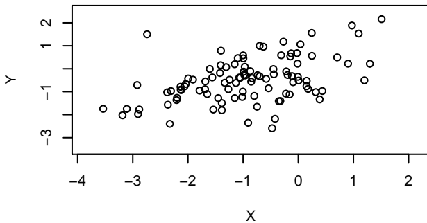
Correlation 0.45
