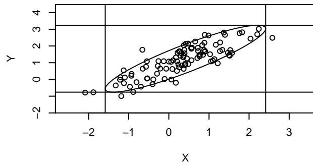
Correlation 0.9
