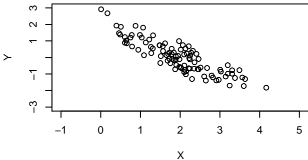
Correlation ??
