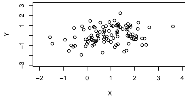
Correlation ??
