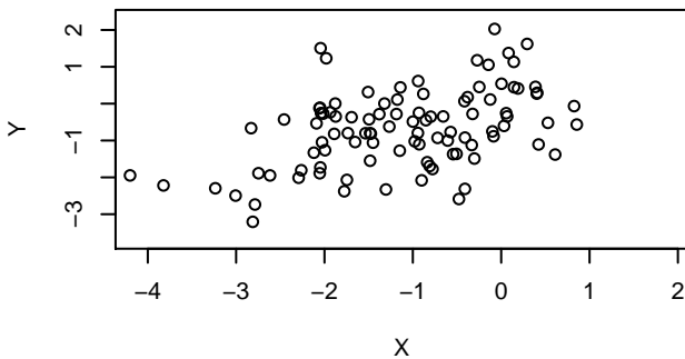
Correlation ??
